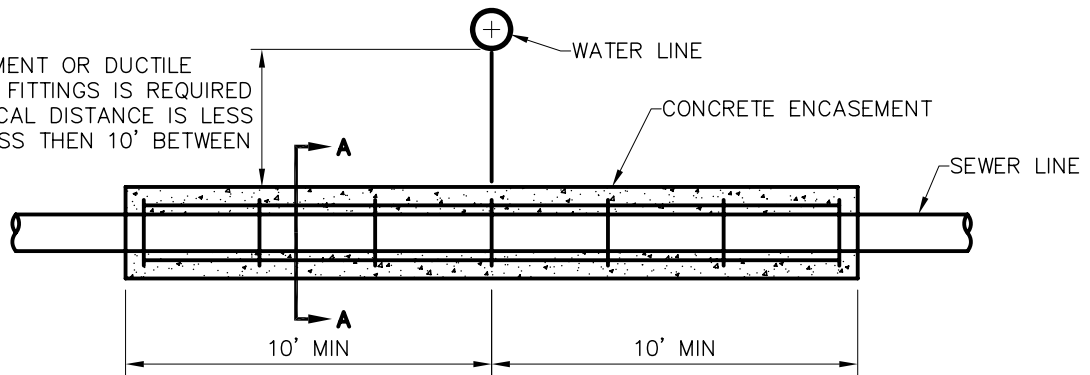
STANDARD UTILITY LINE CROSSING DETAIL
