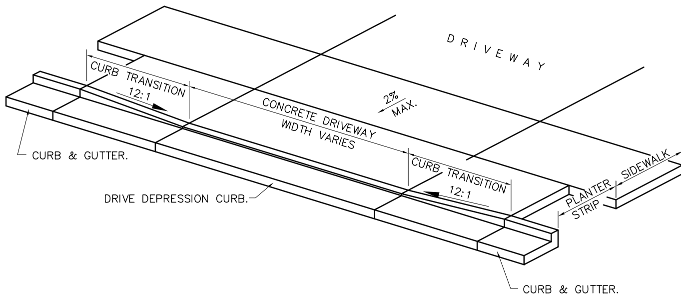
DRIVE DEPRESSION & TRANSITION DETAIL (SIDEWALK WITH PLANTER STRIP)
