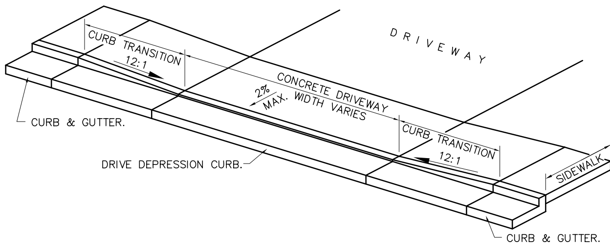
DRIVE DEPRESSION & TRANSITION DETAIL (DIPPED SIDEWALK)
